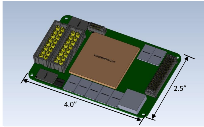
Figure 7 – Pentek's QuartzXM eXpress Module
