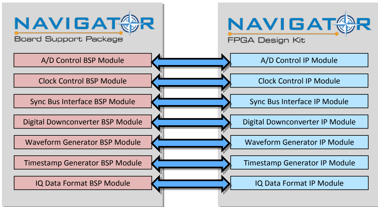
Figure 10 – Navigator’s one-to-one relationship between BSP modules and IP modules simplifies the task of keeping software changes synchronized with IP changes
