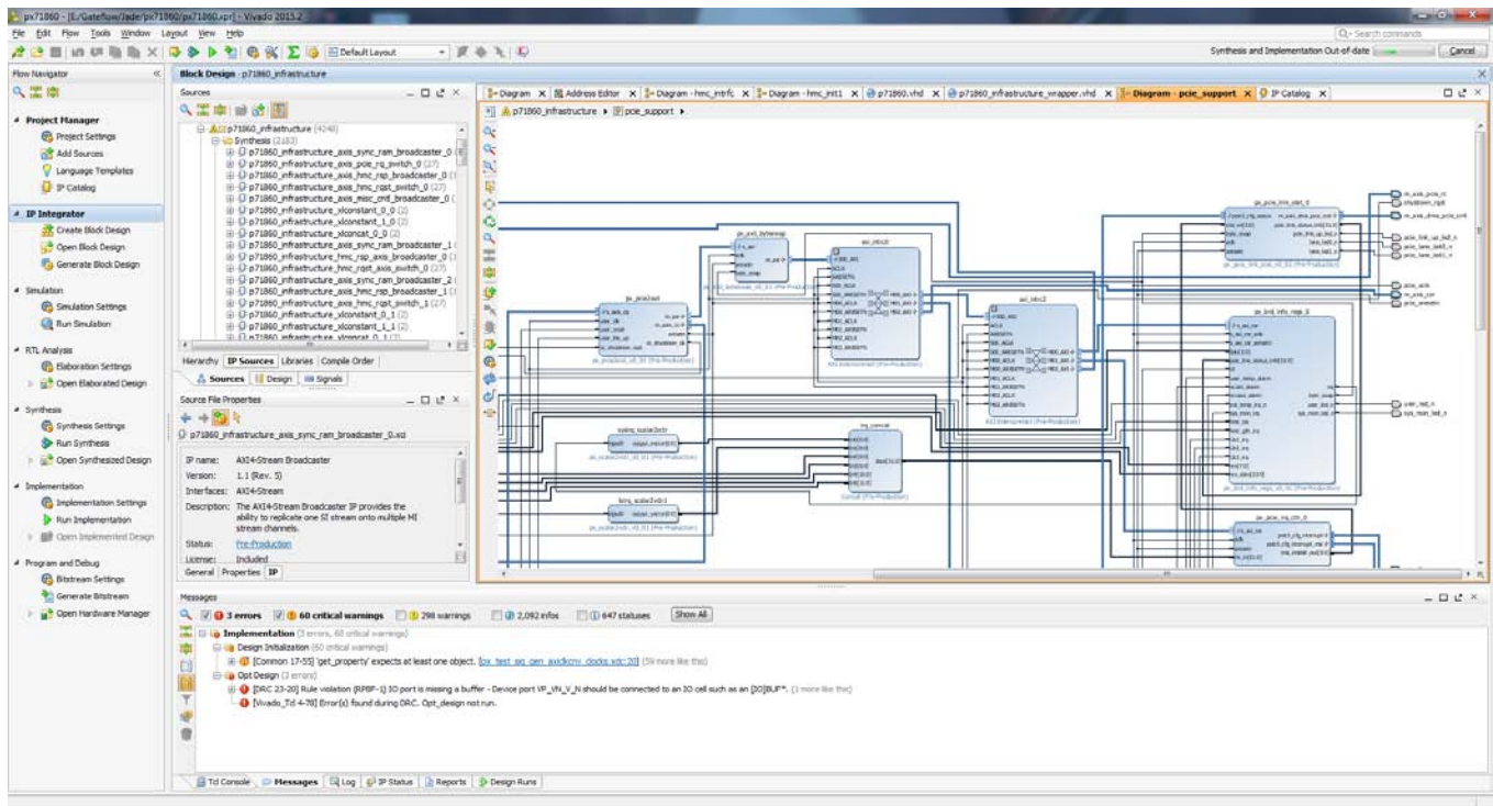
Figure 9 – Pentek's Navigator FDK allows FPGA engineers to access the board design in IP Integrator
