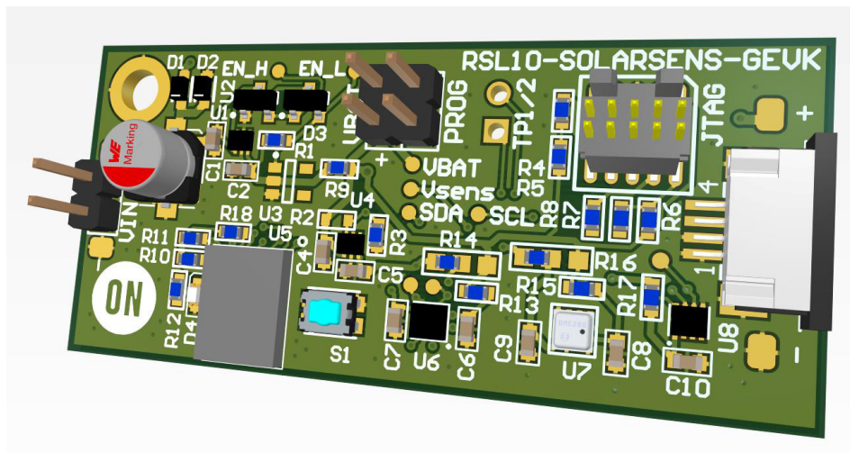
Figure 13. RSL10 Solar Cell Multi-Sensor Board
